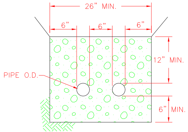
TYPICAL SERVICE TRENCH
