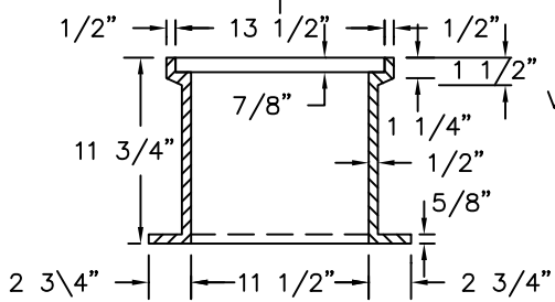
SECTION ON CENTER OF FRAME
