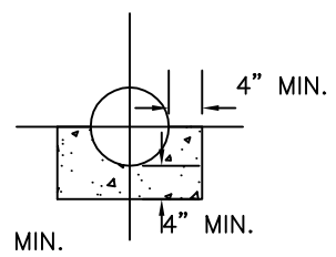
SECTION C-C
